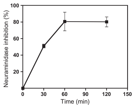
Fig. 3. NA inhibition by gNO. H1N1 was dried on a glass slide and exposed to 160 ppm gNO. Controls were exposed to air. NA inhibition was measured using a commercially available kit and presented as percentage of control following 30, 60, 120 min of gNO exposure.
