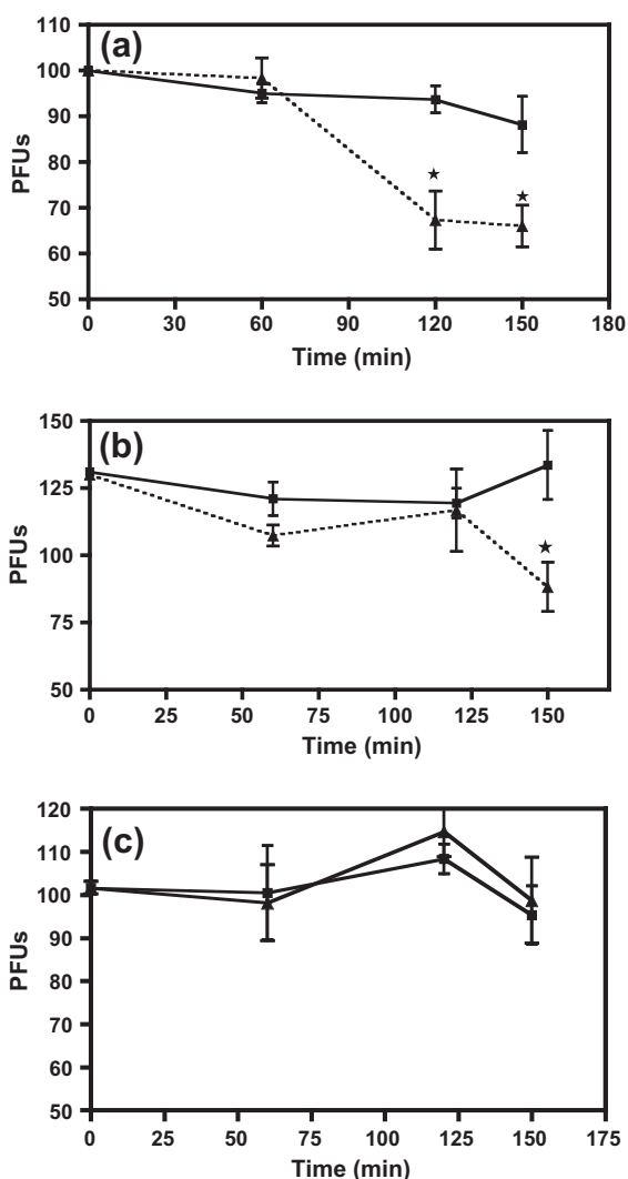
Fig. 1. Post infection inhibition effect of gNO on influenza virus. (a) H1N1, (b) H3N2, (c) Influenza B. Confluent monolayers of MDCK were infected with virus at 100 PFU/well. The plates were continuously shaken on a shaker for 45 min at room temperature for virus adsorption. The solution was removed and replaced with 1 ml of saline per well. Infected plates were treated at 160 ppm gNO for 1, 2 and 2.5 h. At the end of each time point, virus infectivity was measured using plaque reduction assay. Squares represent control (air) while triangles represent gNO exposure. Error bars indicate the standard deviation for two sets of triplicates.
